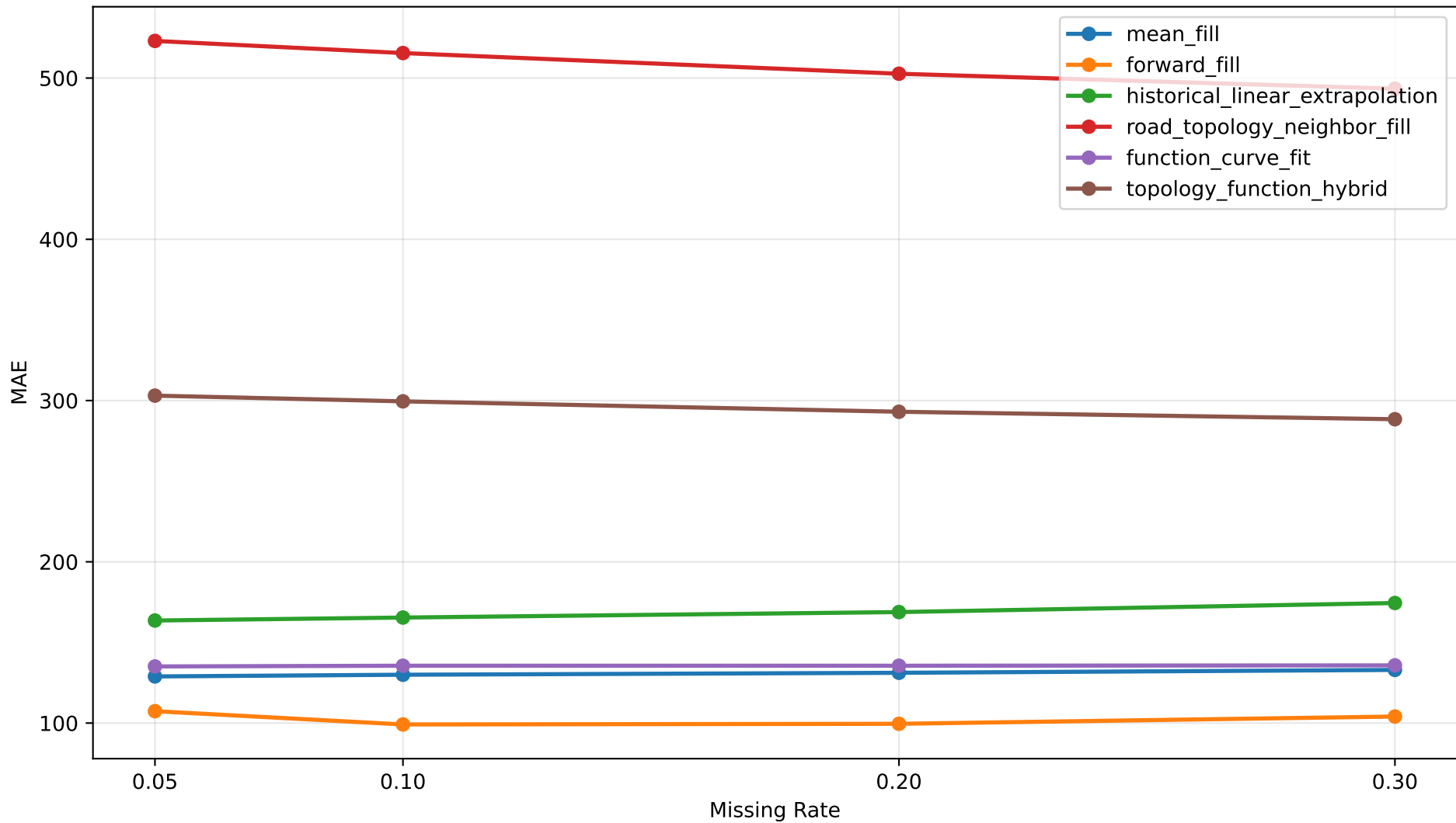
Structured Node Subset Outage MAE by Method
