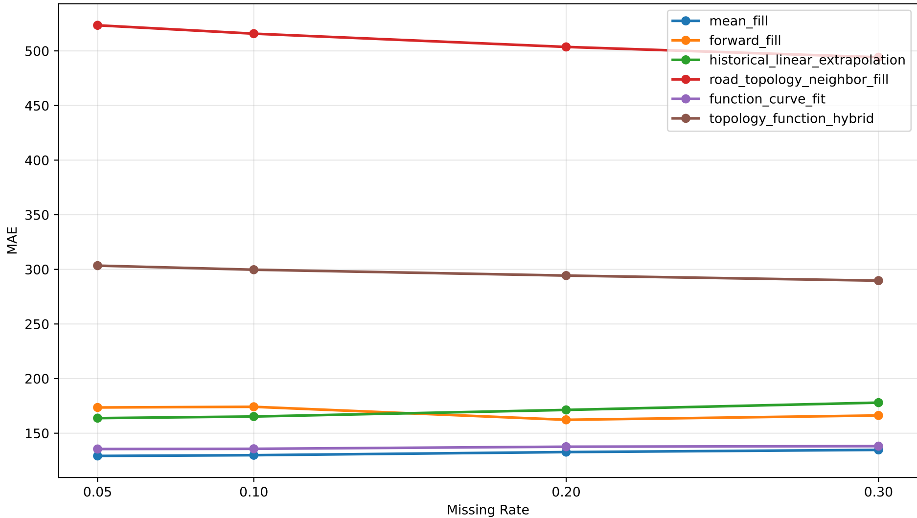
Structured Temporal Block MAE by Method
