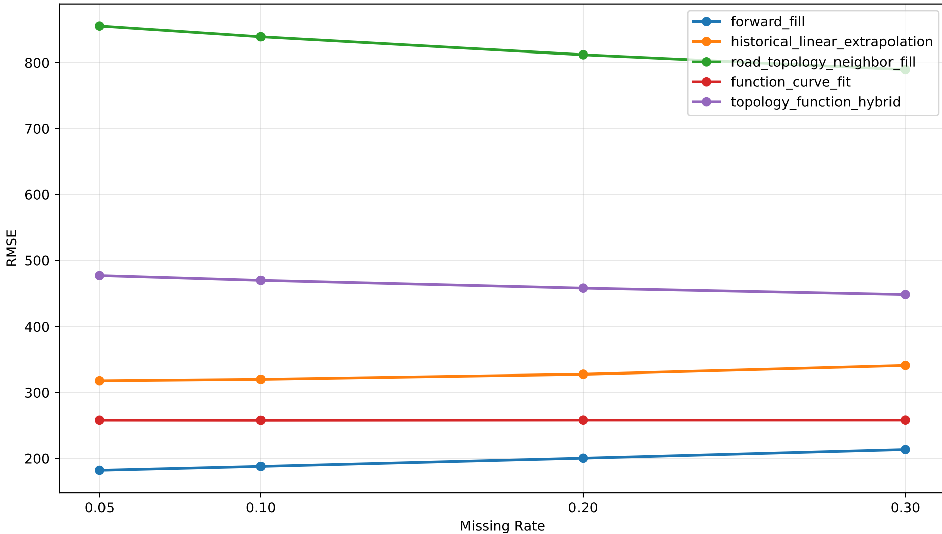
Global MCAR Imputation RMSE by Method (Non-Zero Methods Only)
