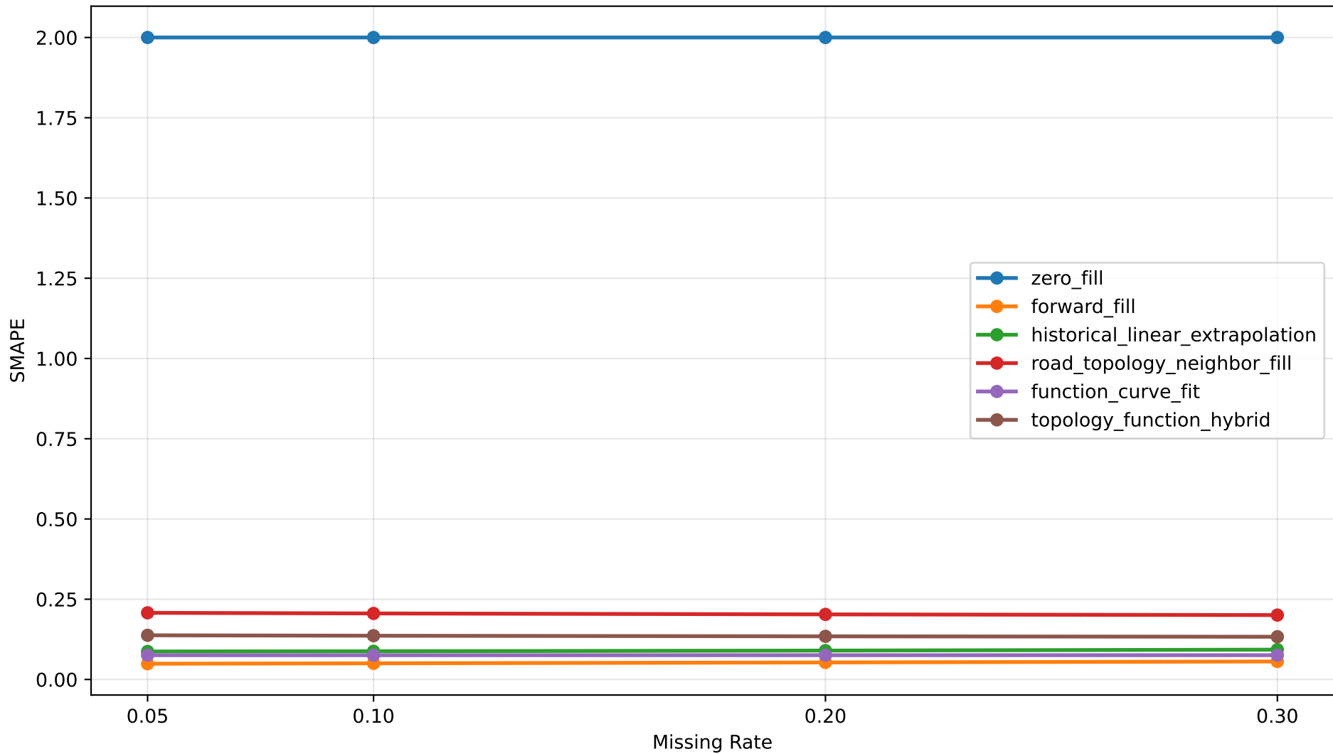
Global MCAR Imputation SMAPE by Method
