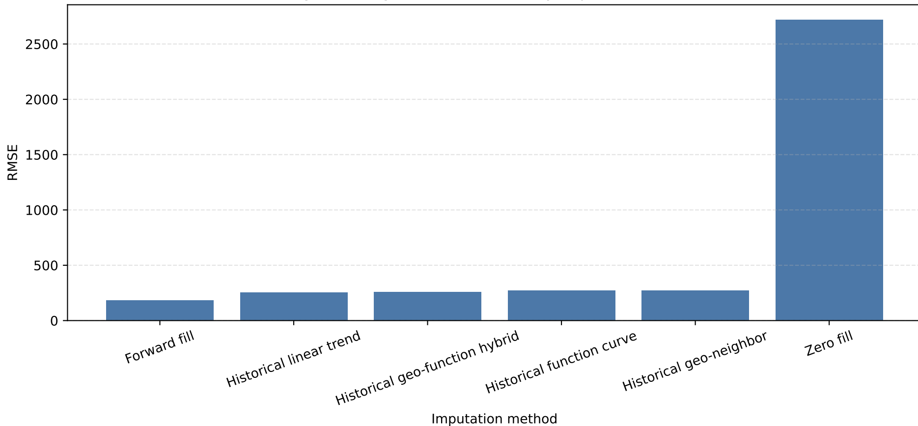
Single missing rate = 5%: RMSE by imputation method
