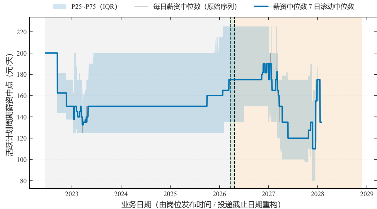
(a) 活跃计划周期薪资中位数与 IQR (Strict 口径)
