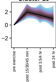
Cluster 10
