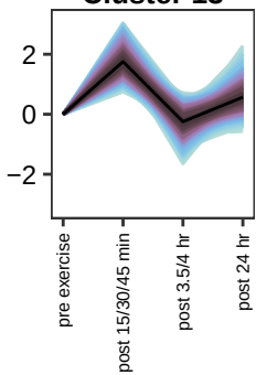
Cluster 13
