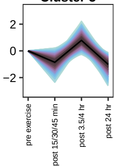
Cluster 9
