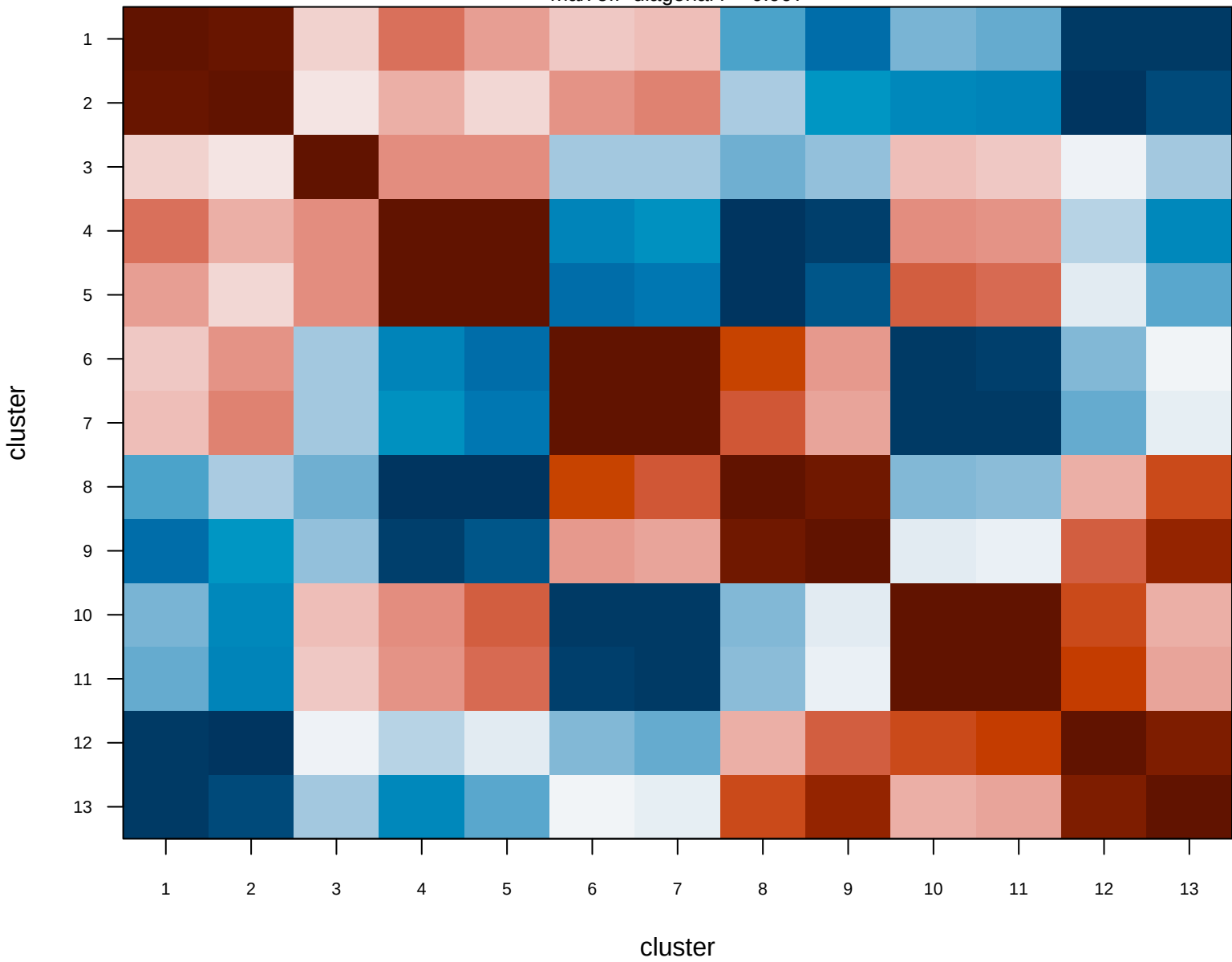
max off-diagonal r = 0.997
