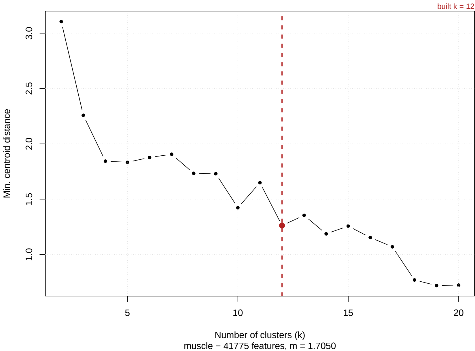
Min. centroid distance (elbow is better)
