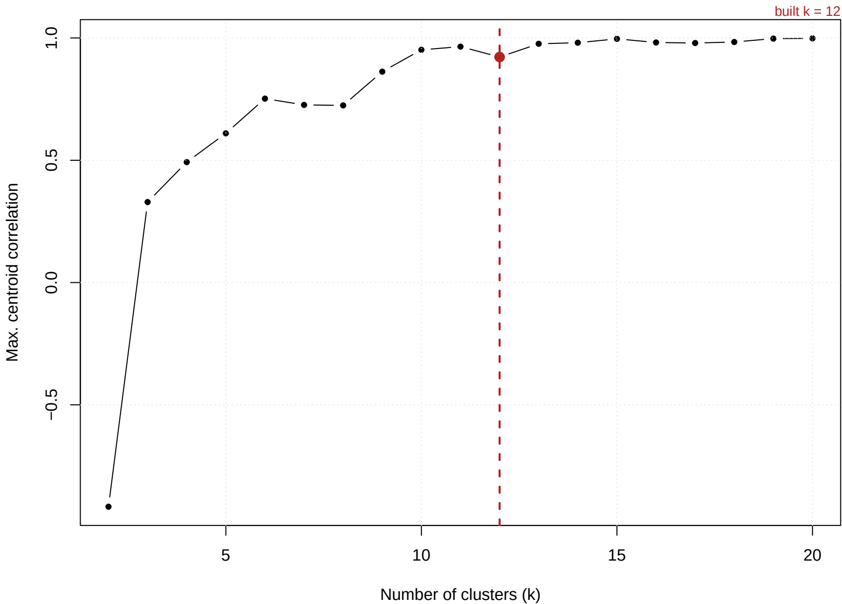
Max. centroid correlation (lower is better)
