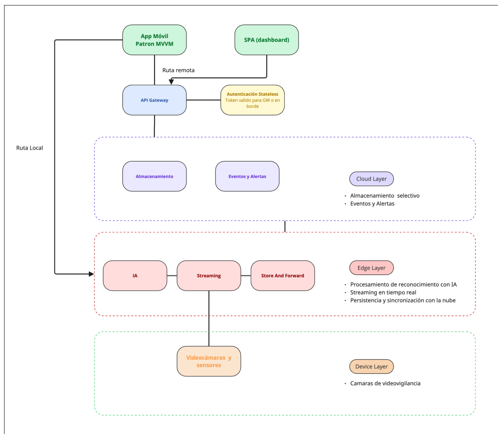
Figure 4: Arquitectura Edge Computing instanciada
