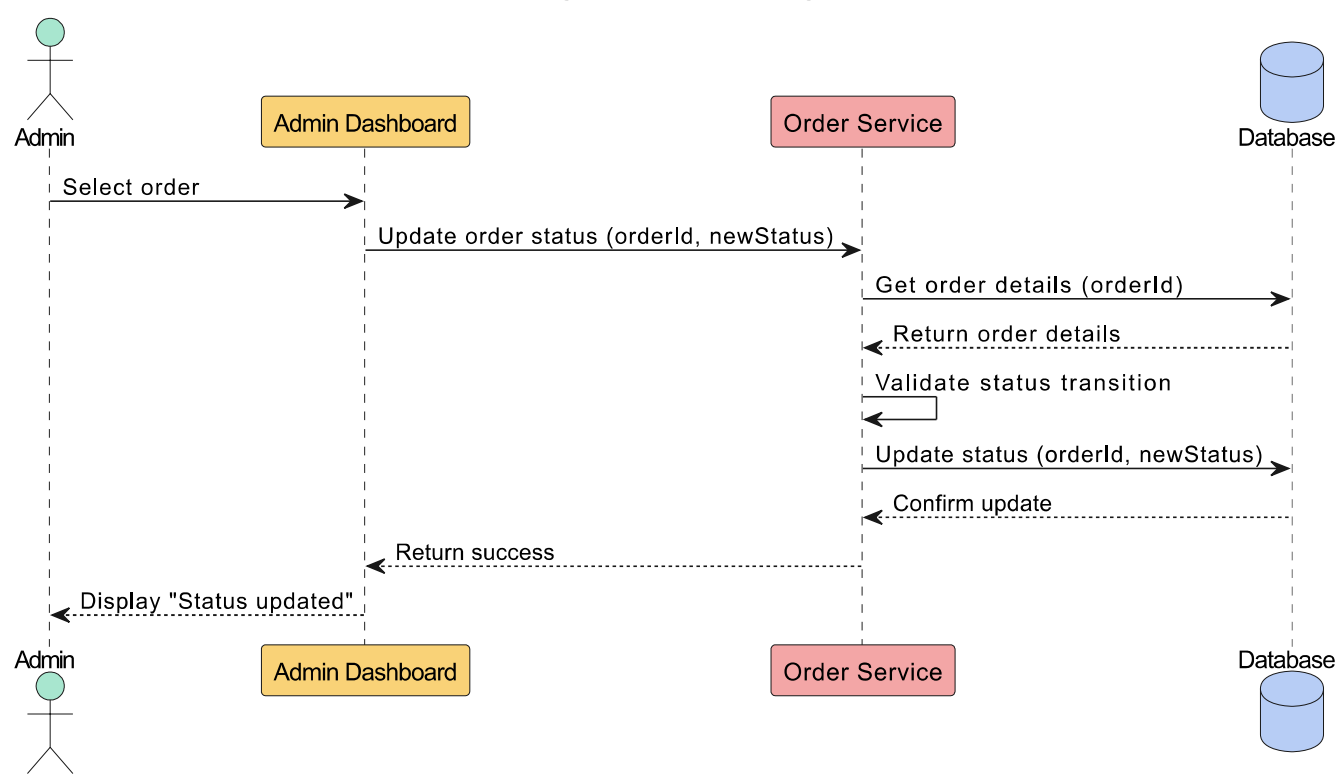
Manage Order Sequence Diagram
