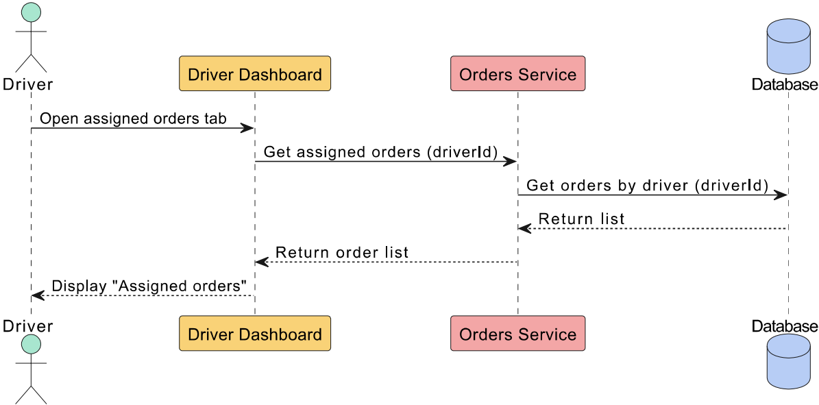
View Assigned Order Sequence Diagram
