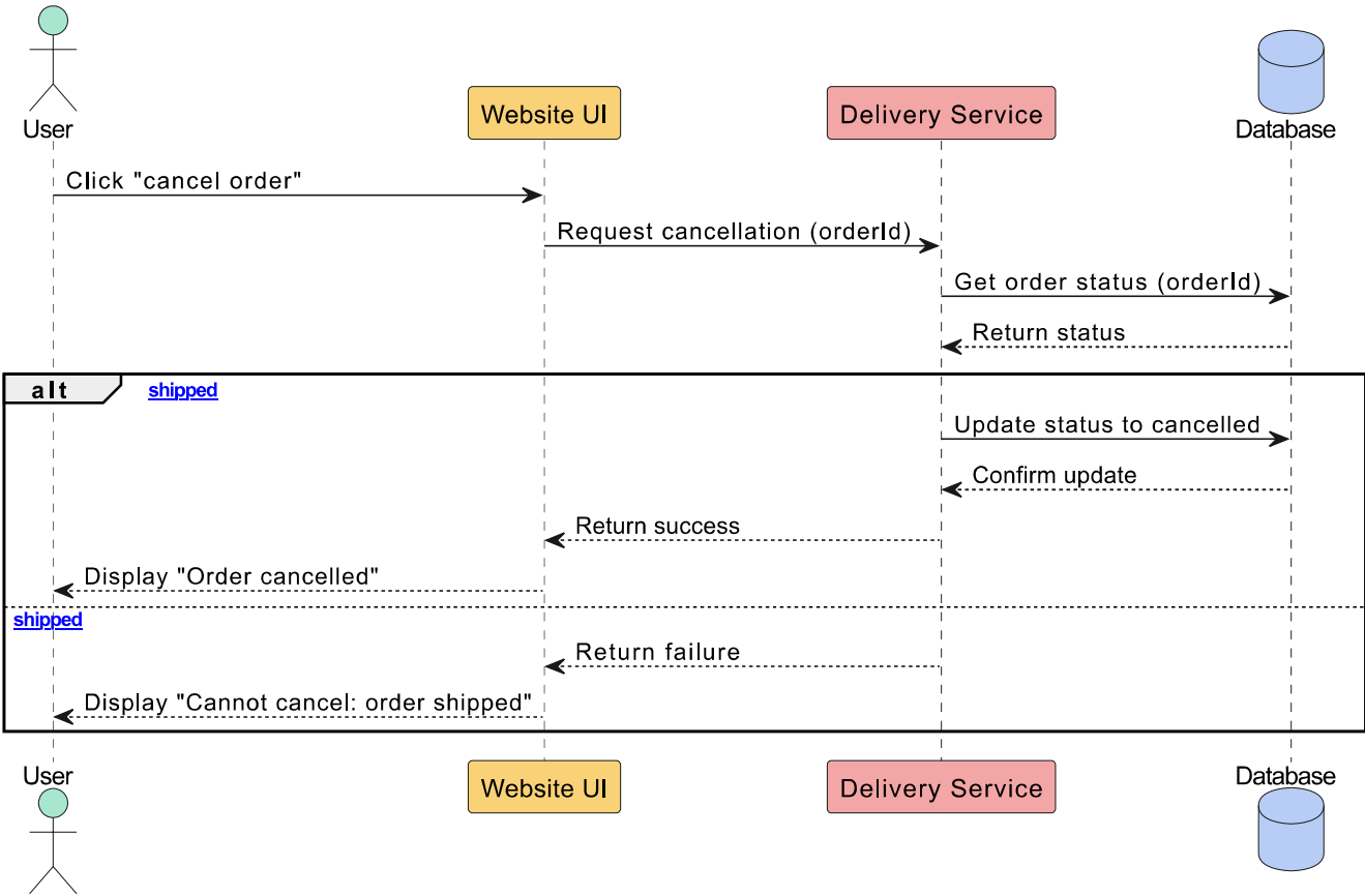
Cancel Order Sequence Diagram
