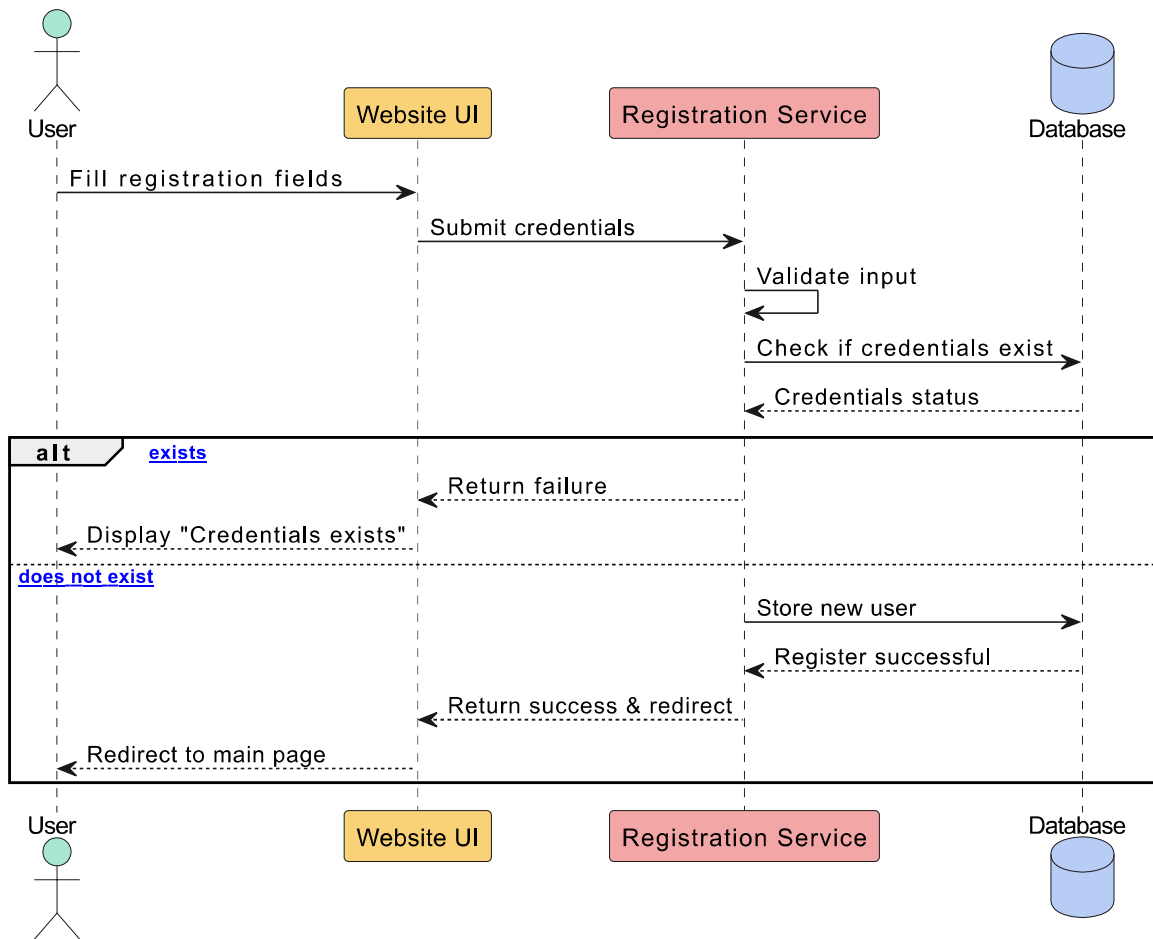
Registration Sequence Diagram
