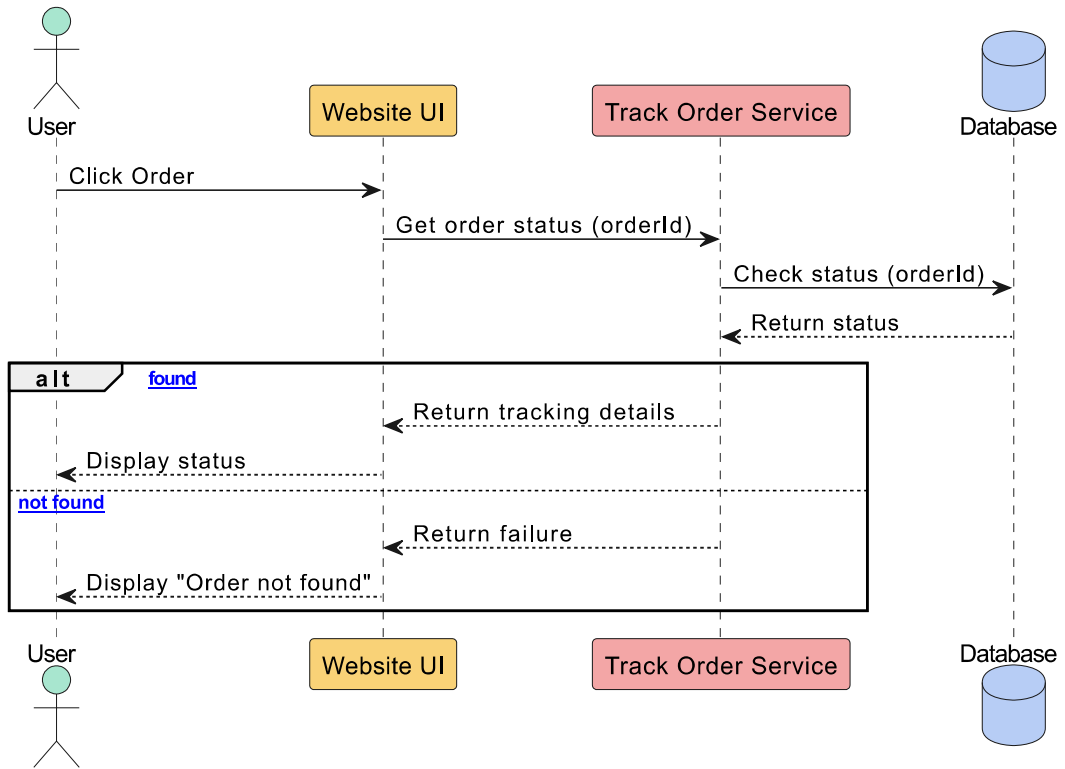
Track Order Sequence Diagram
