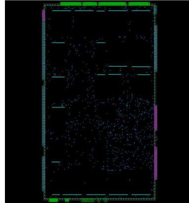
Global route congestion map
