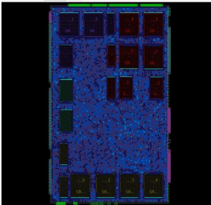
Pin density map
