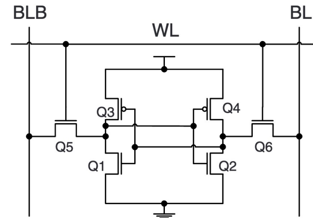
SRAM unit Cell
