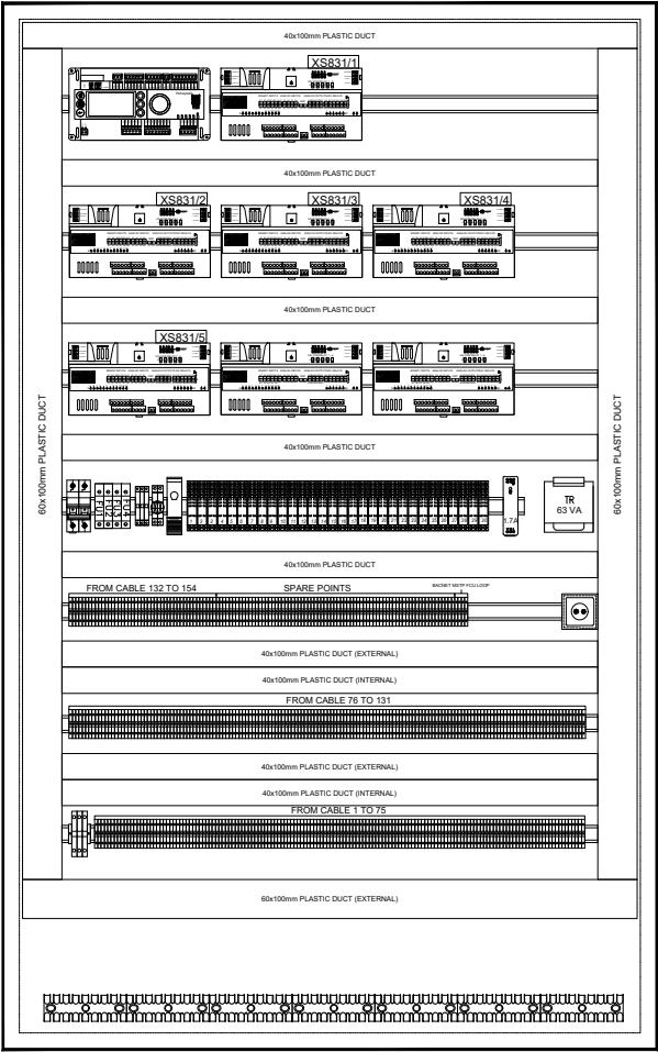
↑ Bottom Entry ↑ Panel Front View Without Door
