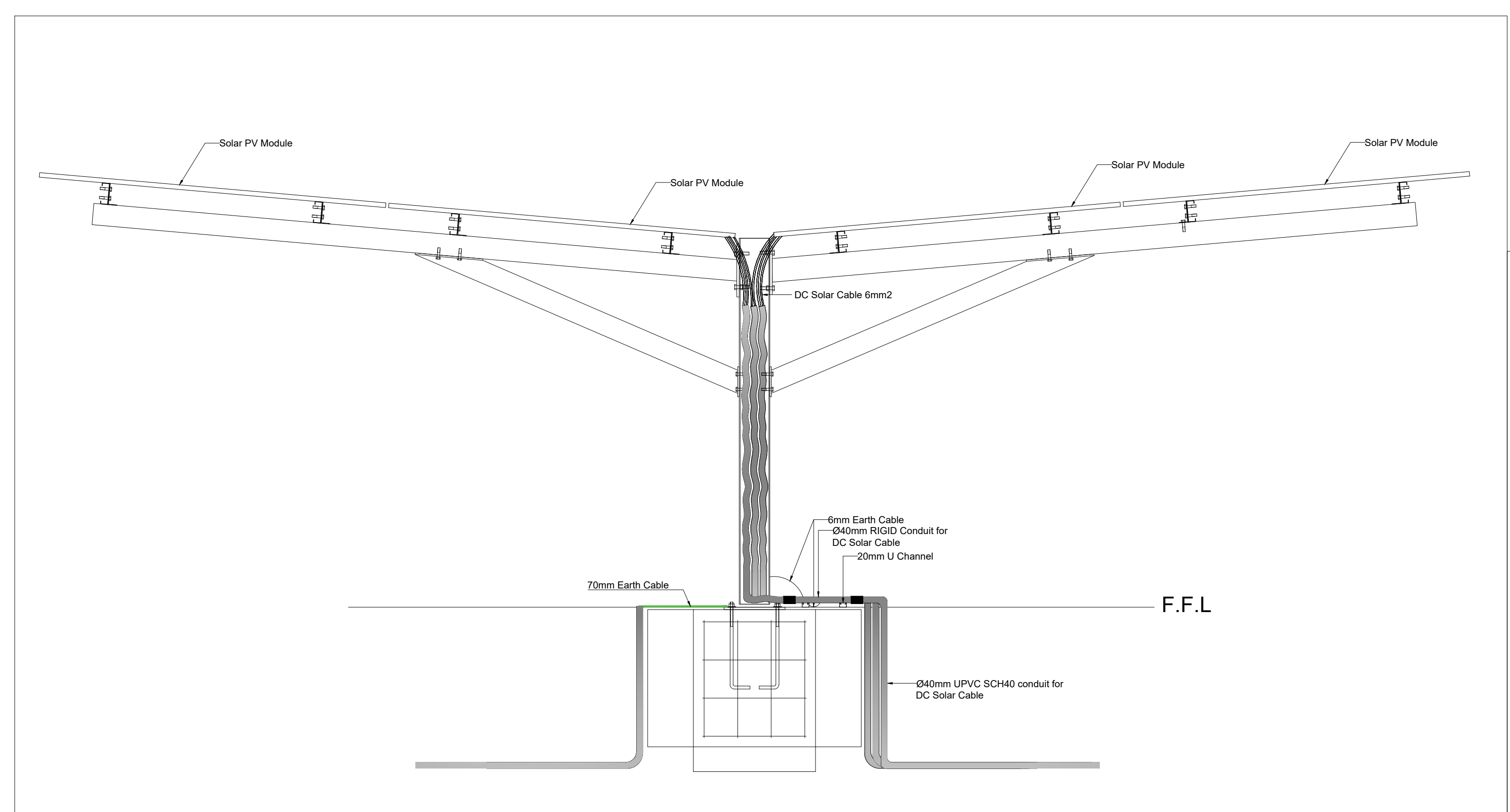
Typical detail for DC Cables Pipes installation Into Car Port
