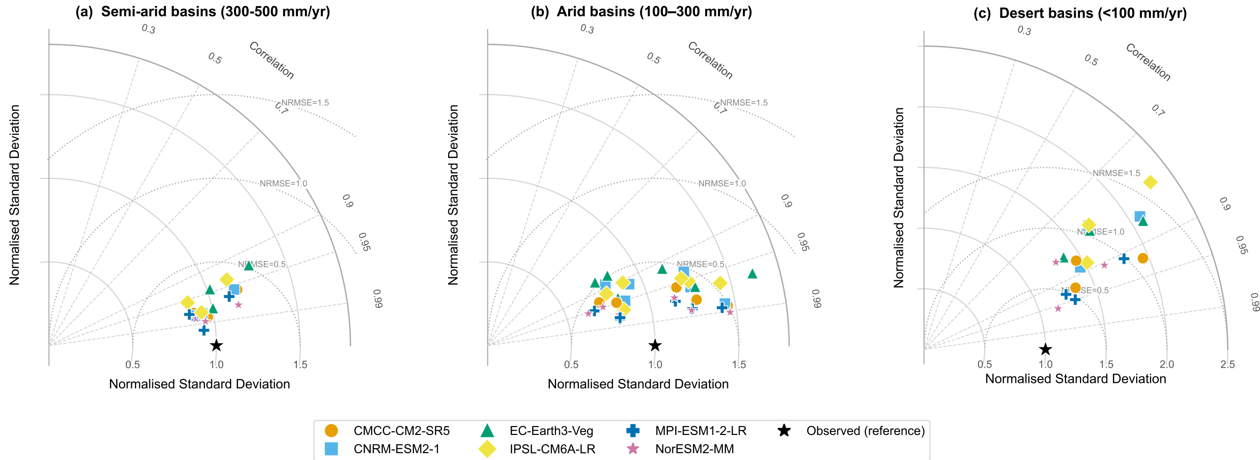
Taylor diagrams for six CMIP6 models across Jordan's basins stratified by aridity class (1995–2014).
