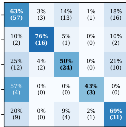
(b) MMD
