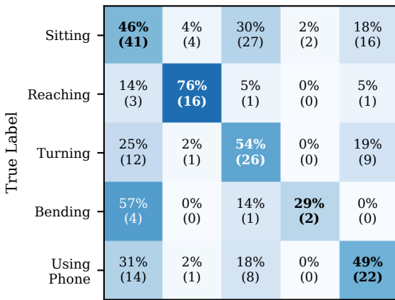
(a) Transfer (No DA)
