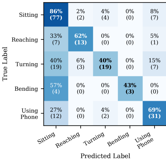
(c) DRCA
