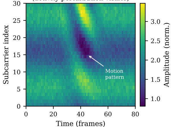
(b) CSI amplitude matrix (activity perturbation visible)
