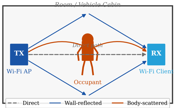
(a) Multipath propagation perturbed by occupant
