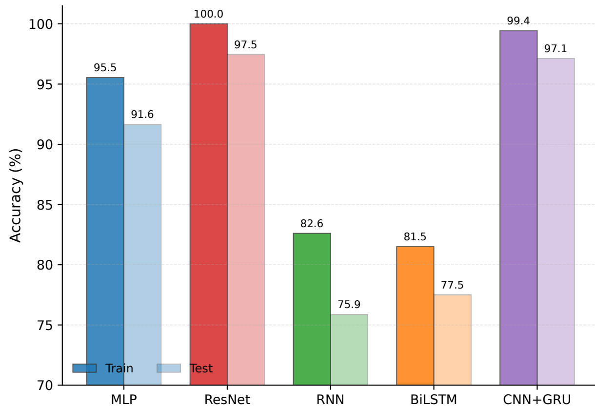
(a) UT-HAR Accuracy (Train vs Test)
