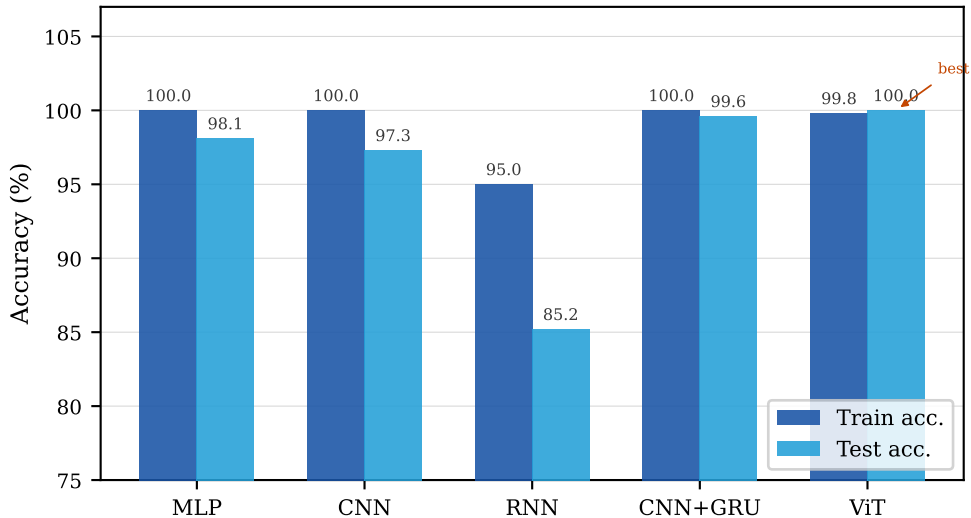
(b) NTU-Fi HAR (6-class, supervised)
