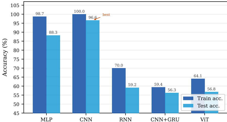
(c) NTU-Human ID (14-subject, SSL fine-tune)
