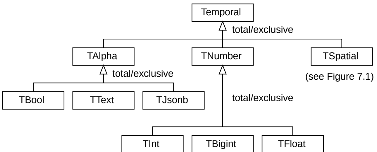
Figure 4.1: Hierarchy of temporal types in MobilityDB.
