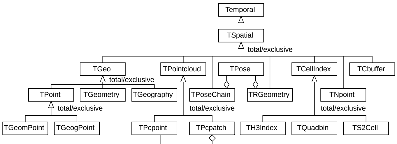
Figure 7.1: Hierarchy of spatiotemporal types in MobilityDB.
