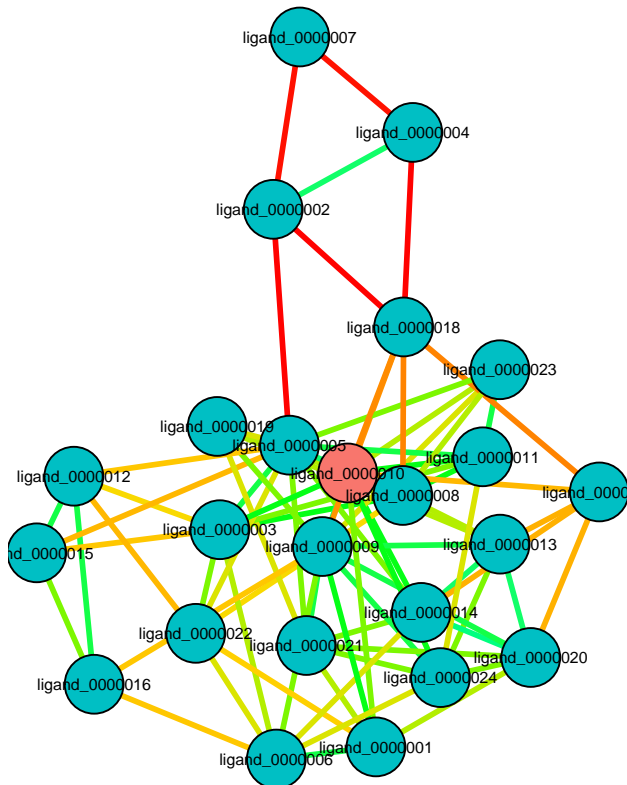
D –optimal
