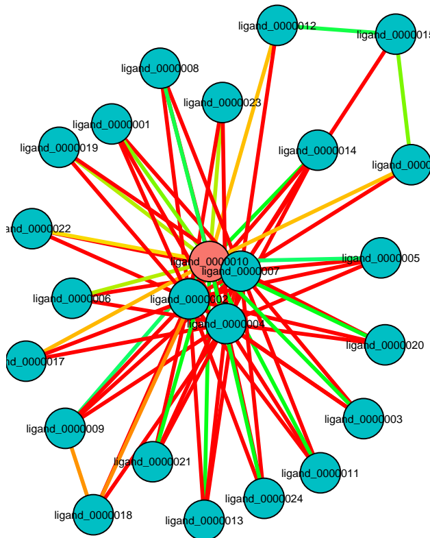
A –optimal
