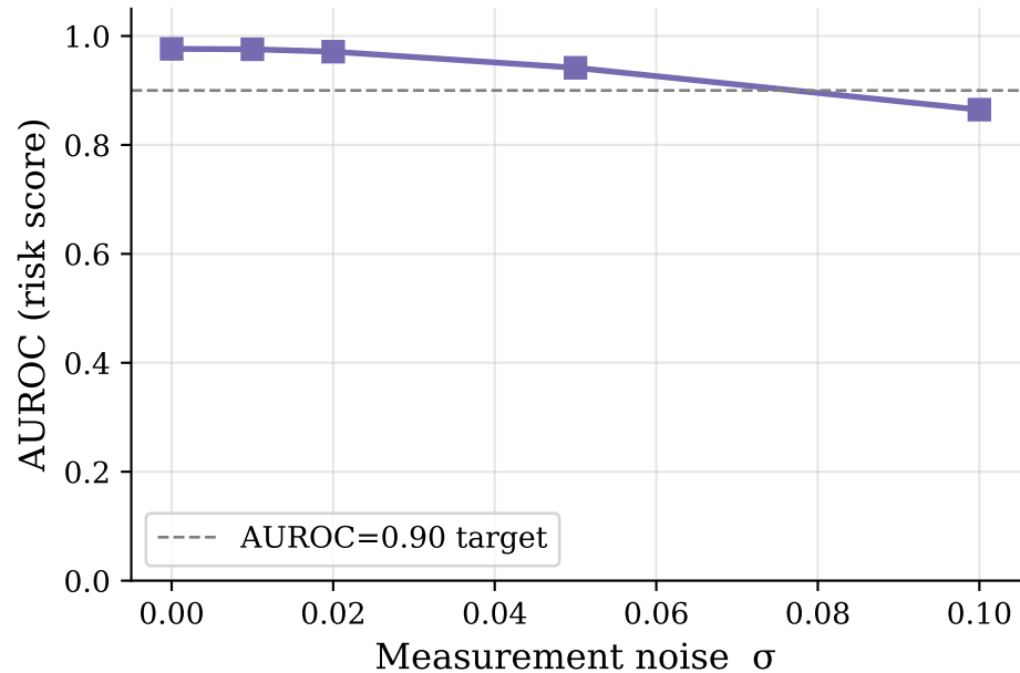
Risk AUROC vs. noise level
