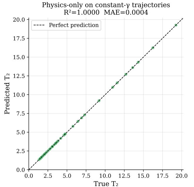
Figure 1: Illustrative validation of the OLS-slope formula (Eq. 2) on 60 fresh constant- \gamma trajectories, independent of the E1 test set (scenario A, Table 4 reports R^2 = 0.9995 on the held-out E1 split; this demonstration set gives R^2 \approx 1.0000 ).
