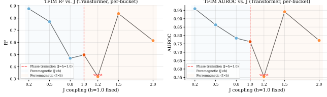
Figure 5: E7c: Transformer R^2 and AUROC trained and evaluated at fixed J values across the TFIM phase diagram ( h = 1.0 fixed). Shaded regions: paramagnetic ( J < h , blue) and ferromagnetic ( J > h , orange). The dashed red line marks the quantum phase transition.
