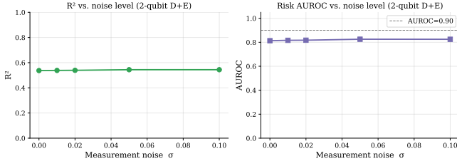
Figure 8 — E6b: 2-qubit noise robustness (physics_lstm, 500 trajs)
