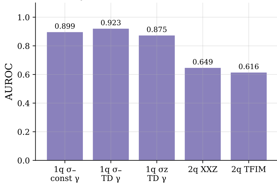
Cross-system AUROC (mixture-trained model)
