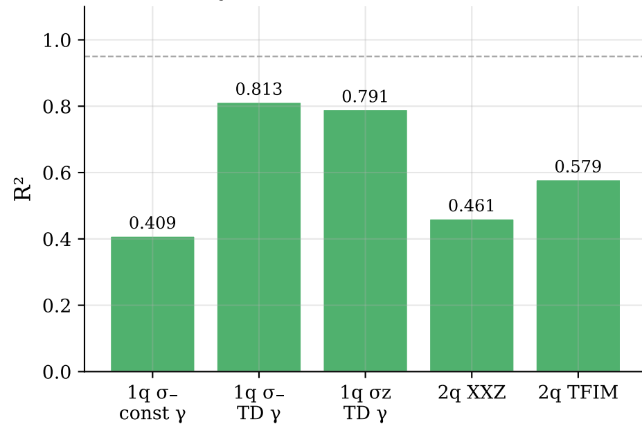
Cross-system R^2 (mixture-trained model)
