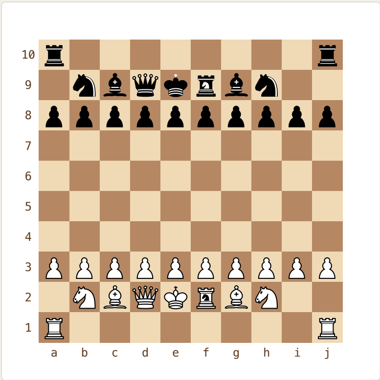
Grand Chess — starting position (10×10)
