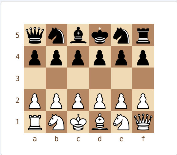
Petty Chess — starting position (5×6)
