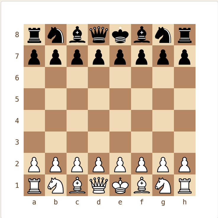
Hoppe-Poppel — starting position
