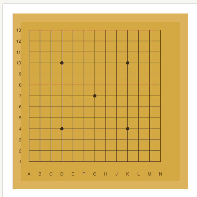
Go — 13×13 board
