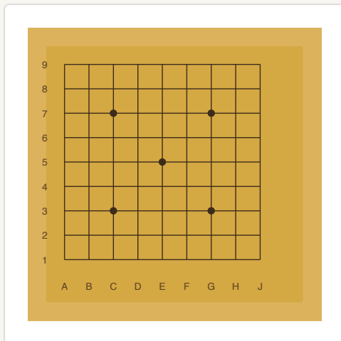
Go — 9×9 board
