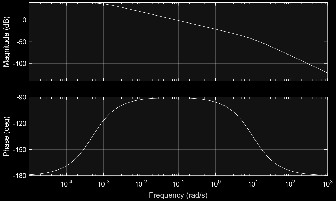
Initial Bode Diagram - Yaw axis
