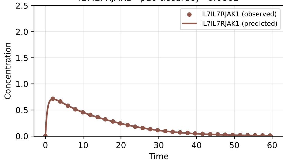
IL7IL7RJAK1 p10 accuracy=0.6862
