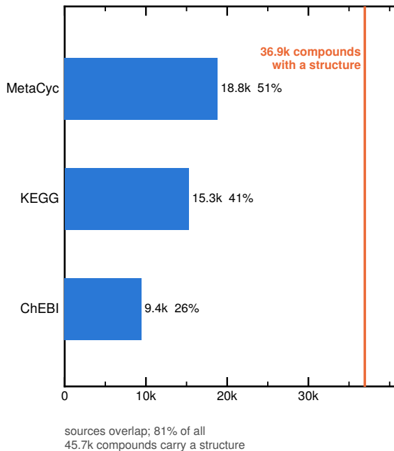
B Structures reaching ModelSEED compounds
