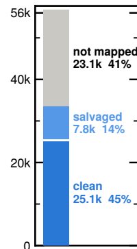
C Atom mapping
