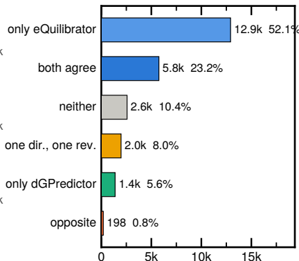
B eQuilibrator vs dGPredictor
