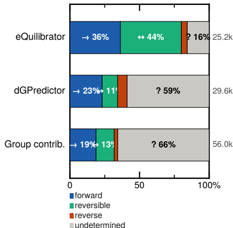
A Direction by source
