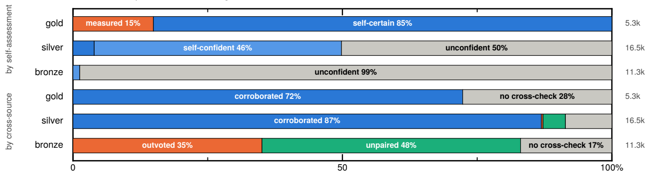
D What underpins each evidence grade
