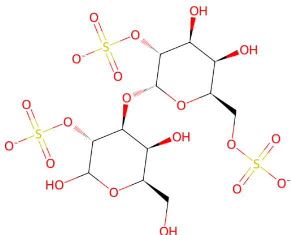
cpd25687 alpha-D-Galp2,6S2-(1->3)-beta-D-Galp2S-(1->4)-alpha-D-Galp2,6S
