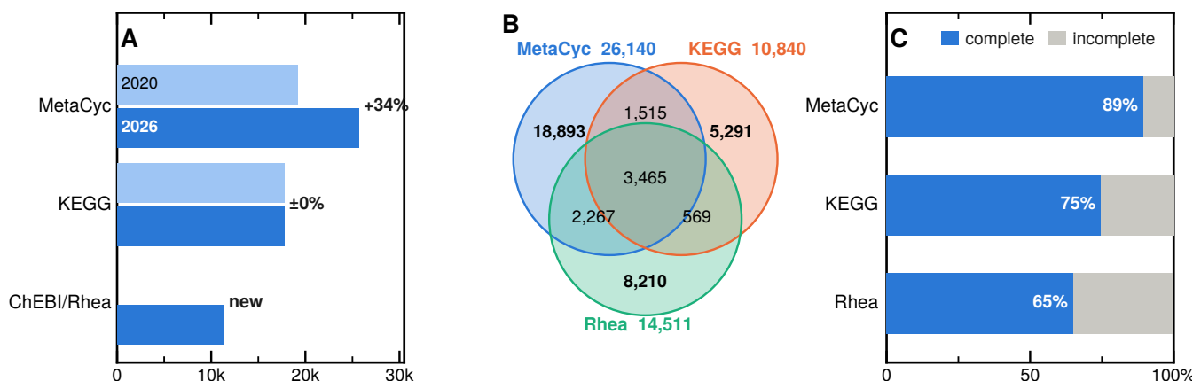
Figure 1 Sources of compounds and reactions, and where the growth landed. Sources of compounds and reactions. (A) compounds contributed by each source that also supplied molecular structures, 2020 against 2026: we did not introduce any new biochemistry from KEGG. The third row is ChEBI, which supplies structures but no reactions. (B) how the three primary reaction sources overlap, every region labelled with its reaction count. Circle areas are not proportional — three-set areas cannot be solved exactly — so the counts carry the quantities and the circles only carry membership . Rhea identifies its compounds through ChEBI. (C) the share of each source's unique reactions that are complete, meaning every reagent is assigned a complete structure, so the reaction can be balanced and decomposed. (D) reactions added since 2020 against those already held, by MetaCyc pathway class, for the eight classes that gained most. Both bars are built through the same join from the MetaCyc source table, so they are comparable; the organisational class Super-Pathways is excluded. Only additions with a MetaCyc pathway assignment can be placed — 2,282 of the 12,259; the 8,409 reactions that arrived through Rhea carry no pathway ontology and are absent from the panel rather than counted as unannotated. Growth is concentrated in specialised metabolism and cell-envelope biosynthesis: 41 of the 12,259 reactions added fall in a central carbon or energy-metabolism class.
