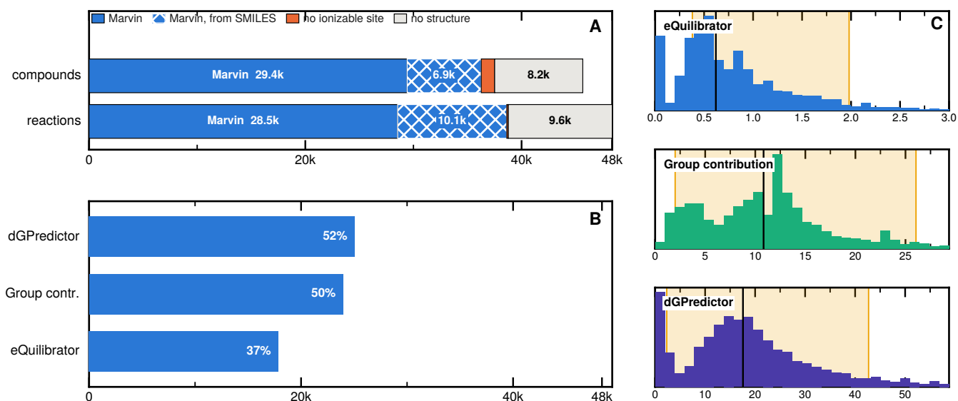
Figure 2 Thermodynamic sources. (A) Provenance of every pK_a ladder shipped in the database, across all 45,662 compounds and 48,384 reactions. ChemAxon Marvin supplies 79.4% of compounds and 79.8% of reactions. Segments are identified by the key. Hatching marks the share reached through a second route: the calculator refuses polymers and organometallics as query molecules, so those are computed from SMILES instead. No ionizable site is a chemistry result — returned by Marvin ran and where it reported no dissociable proton between pH -2 and 16, for 1,237 compounds — and is coloured apart from no structure, which is a curation gap rather than a protonation one. (B) Reactions that carry an energy computed from the source heuristic. (C) Reported uncertainty in \text{kcal mol}^{-1} , one axis per source because the three differ by more than an order of magnitude. The shaded band spans the 5th to 95th percentile, which is used in our classification scheme.
