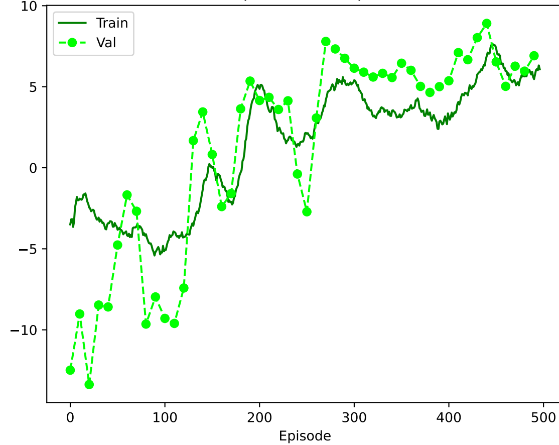
Train vs Val Sharpe (overfitting monitor)
