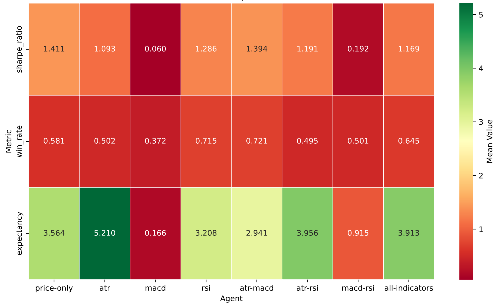
Indicator Ablation Heatmap - Mean Performance
