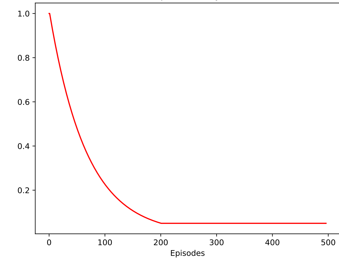
Epsilon Decay
