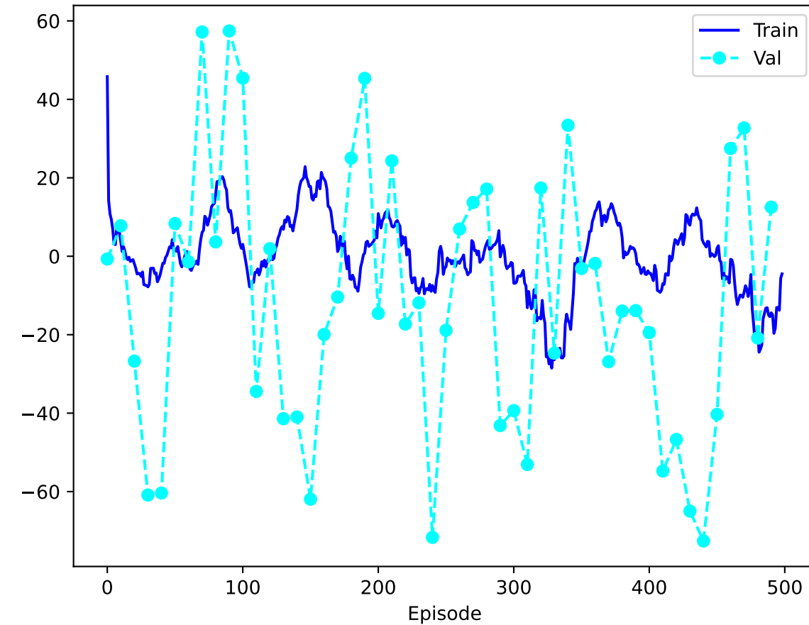
Epsilon Decay
