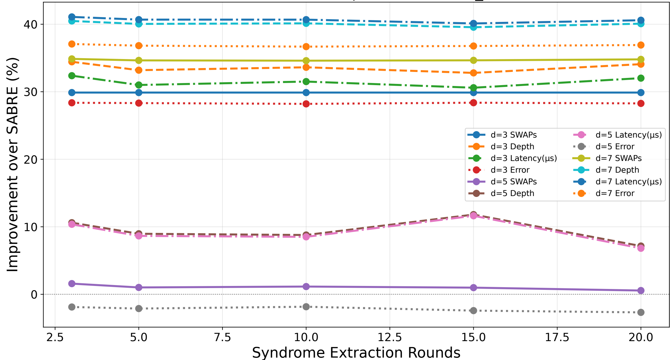
Surface Code: Qlosure Improvement (ibm_brisbane)
