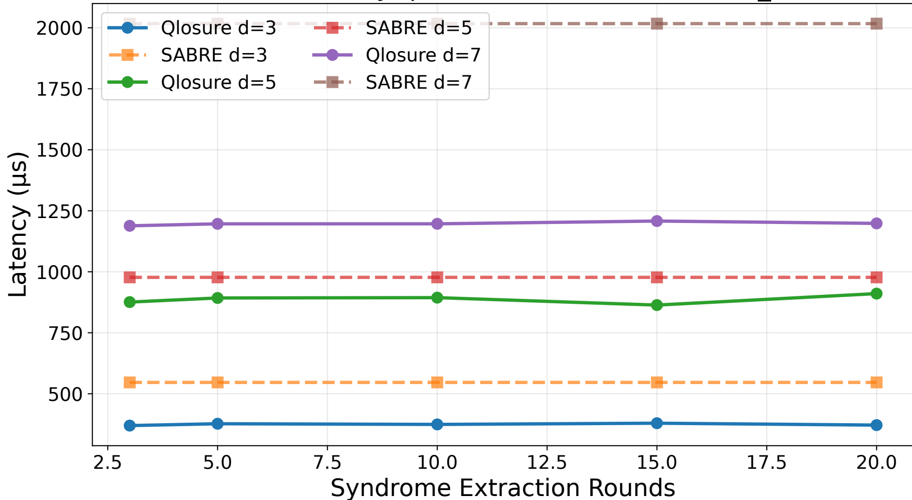
Surface Code Latency ( \mu\text{s} ): Qlosure vs SABRE (ibm_brisbane)
