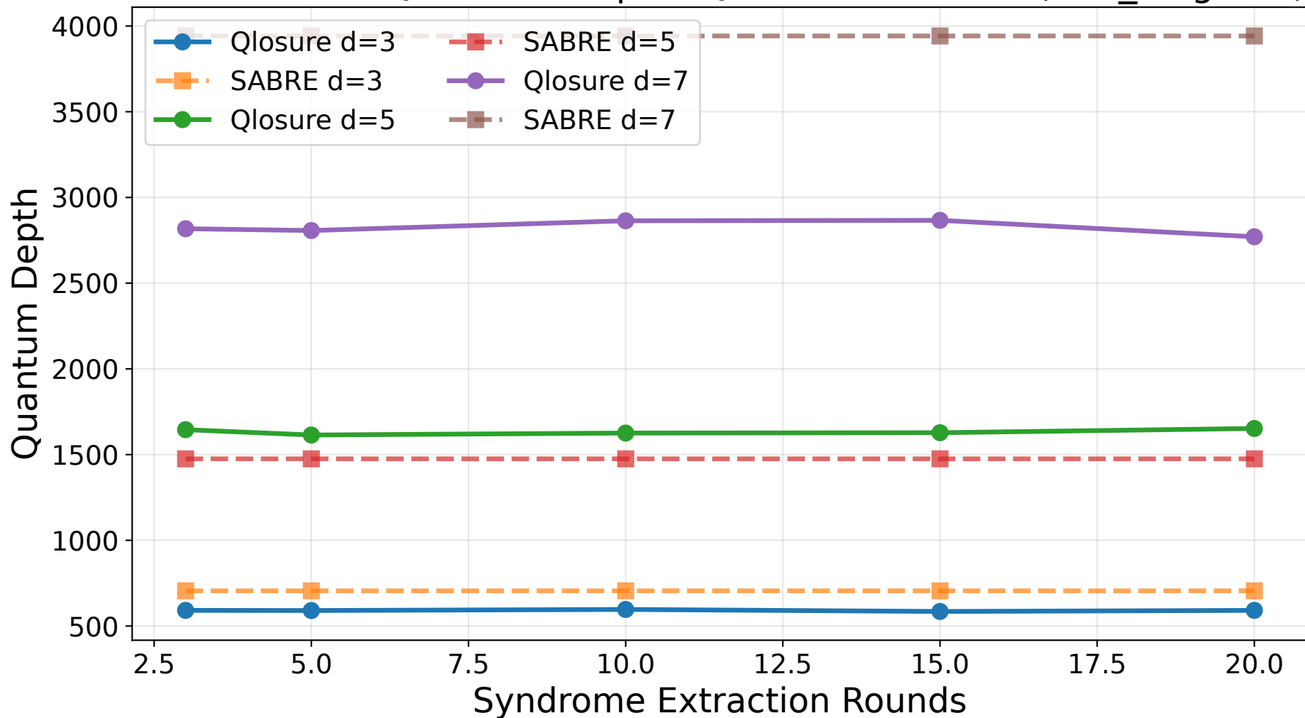
Surface Code Quantum Depth: Qlosure vs SABRE (ibm_kingston)
