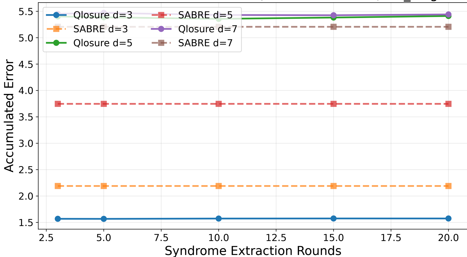
Surface Code Accumulated Error: Qlosure vs SABRE (ibm_kingston)
