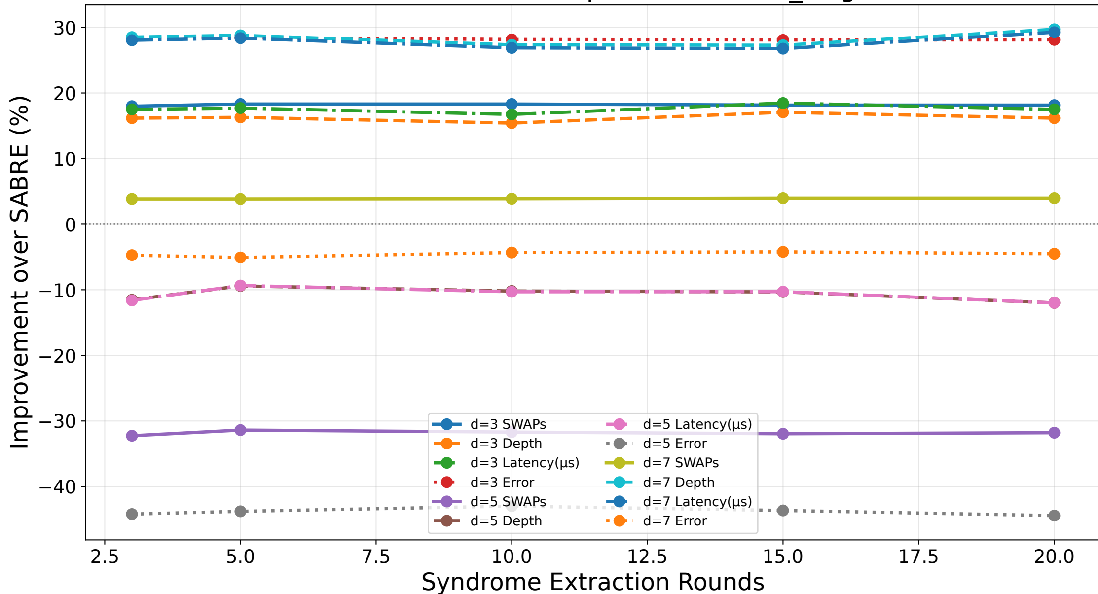
Surface Code: Qlosure Improvement (ibm_kingston)
