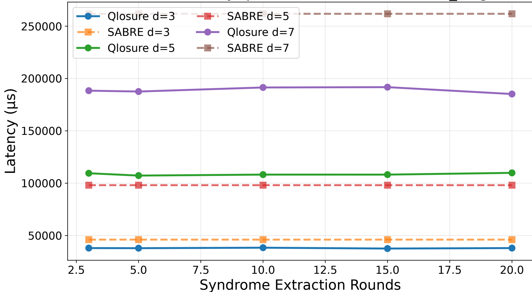
Surface Code Latency ( \mu\text{s} ): Qlosure vs SABRE (ibm_kingston)
