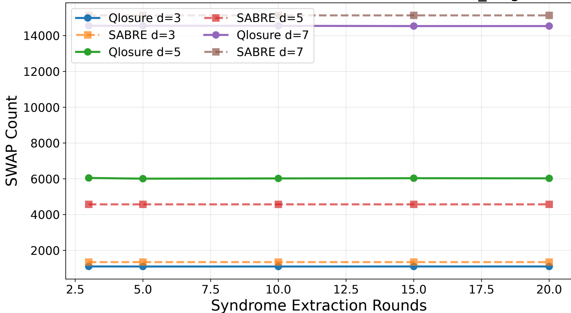
Surface Code SWAP Count: Qlosure vs SABRE (ibm_kingston)
