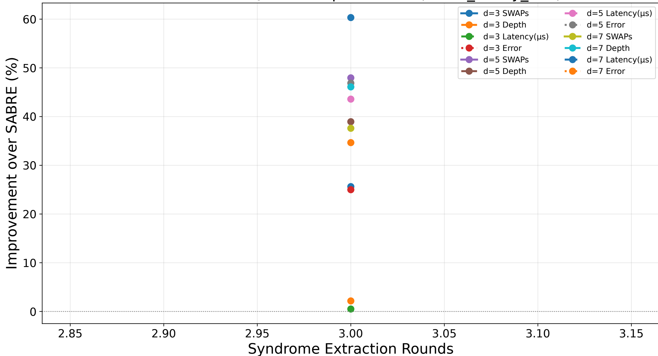
Surface Code: Qlosure Improvement (mech_heavy_hex)
