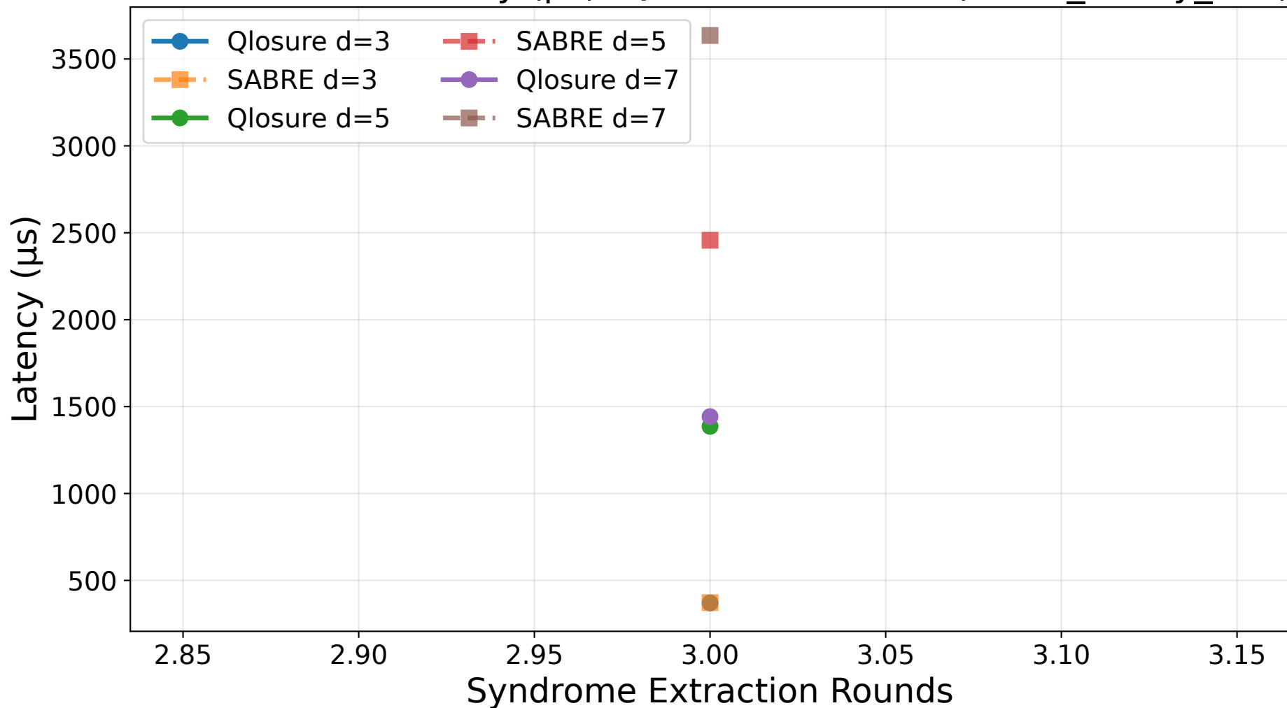
Surface Code Latency ( \mu\text{s} ): Qlosure vs SABRE (mech_heavy_hex)
