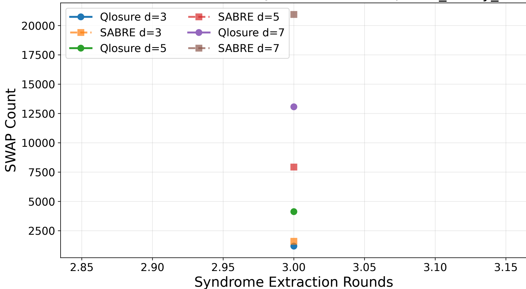
Surface Code SWAP Count: Qlosure vs SABRE (mech_heavy_hex)
