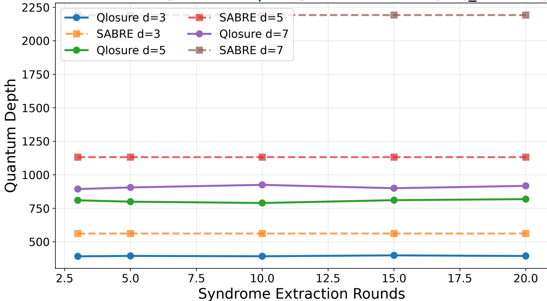
Surface Code Quantum Depth: Qlosure vs SABRE (ibm_brisbane)
